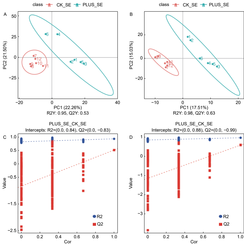
A, C-正离子模式下的 PLS-DA 模型得分散点图及其置换结果检验; B, D-负离子模式下的 PLS-DA 模型得分散点图及其置换结果检验。A, C-PLS-DA scores and the related examination result under positive ionization mode; B, D-PLS-DA scores and the related examination under negative ionization mode
